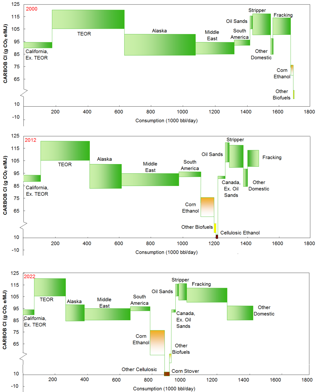
Figure 3.9. Carbon intensity (g CO 2 e/MJ) of petroleum fuels consumed in California
