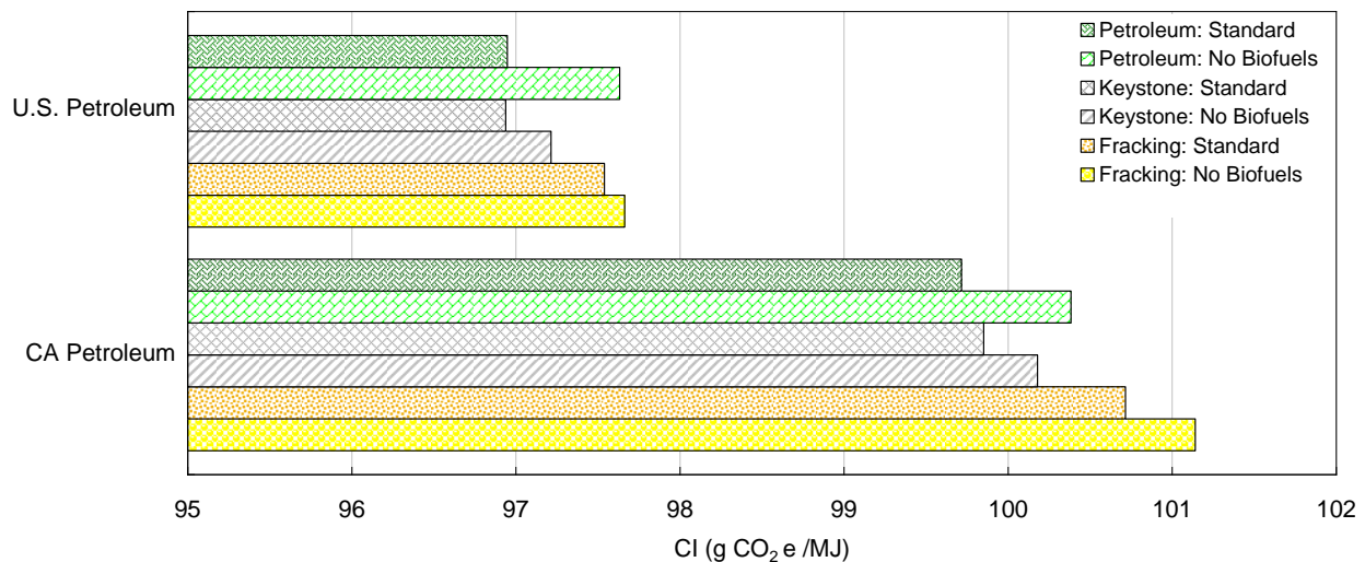
Figure 3.13. Weighted carbon intensity (g CO 2 e/MJ) of petroleum fuels under current projections and alternate likely scenarios.
