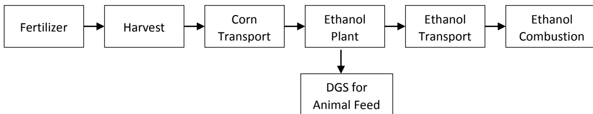
Figure 3.2. Simplified corn ethanol system boundary diagram.
