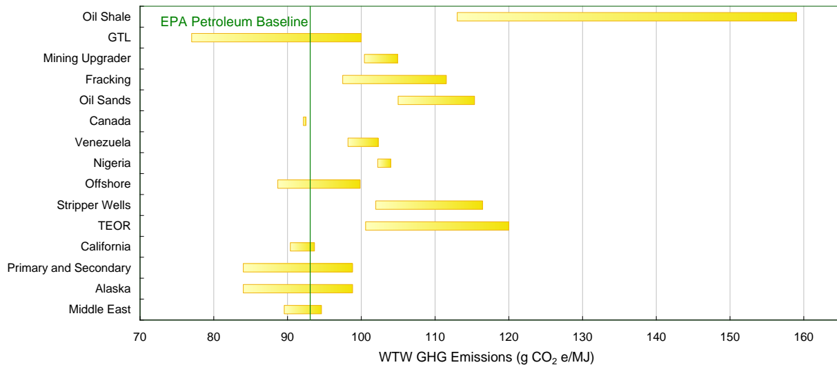
Figure 3.12. Carbon intensity (g CO 2 e/MJ) of petroleum fuels
