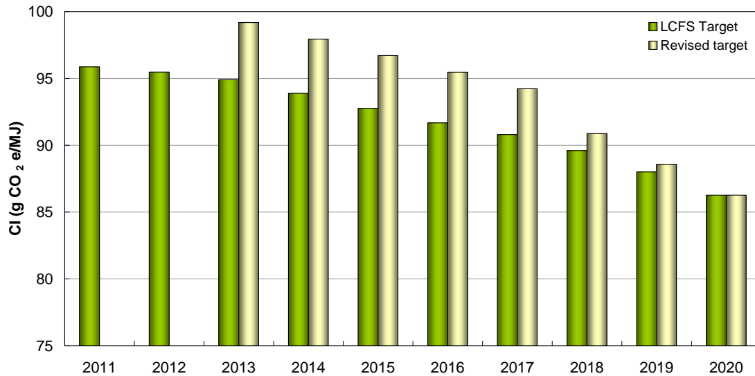
Figure 1.2. California LCFS compliance schedule
