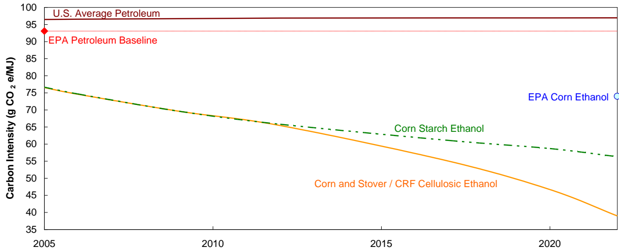
Figure S.1. Carbon intensity (g CO 2 e/MJ) of petroleum gasoline and corn ethanol consumed in the U.S. over time.
