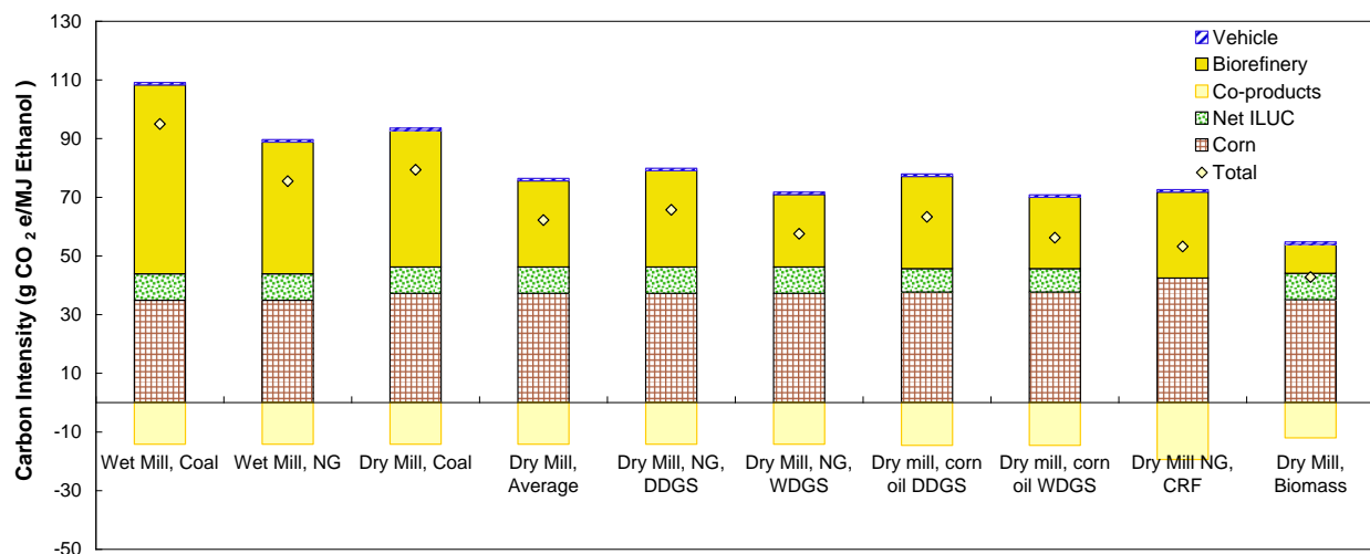
Figure 3.6. Breakdown of the CI emissions (g CO 2 e/MJ) of Corn Ethanol
