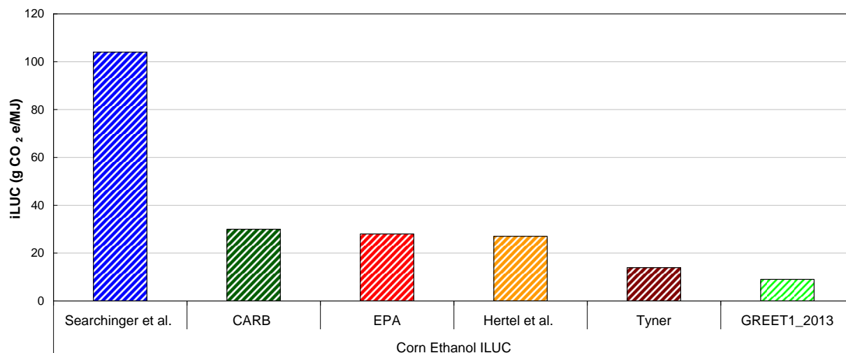
Figure 3.5. Comparison of ILUC from various sources
