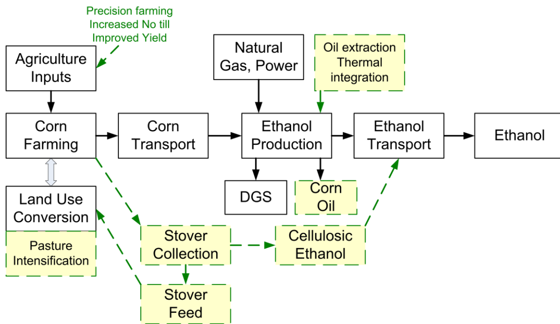
Figure 3.4. Production pathway option for corn ethanol
