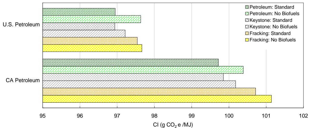
Figure S.2. Weighted carbon intensity (g CO 2 e/MJ) of petroleum fuels under current projections and alternate likely scenarios.
