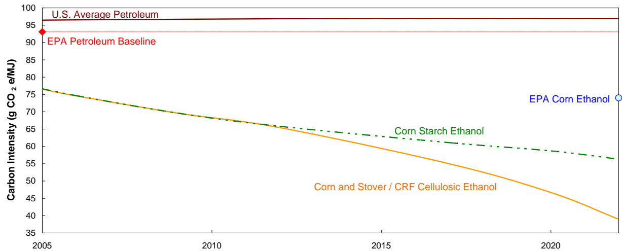
Figure 3.11. Weighted carbon intensity (g CO 2 e/MJ) of petroleum fuels and corn ethanol consumed in the U.S. over time.
