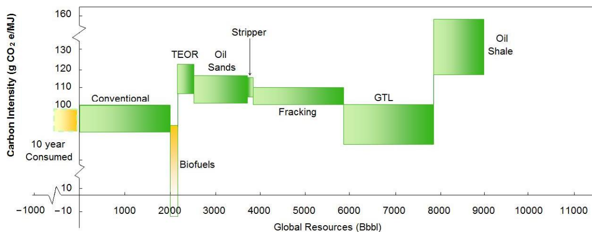
Figure 3.7. Range in of CI of gasoline for different energy resources (g CO 2 e/MJ) (2013)
