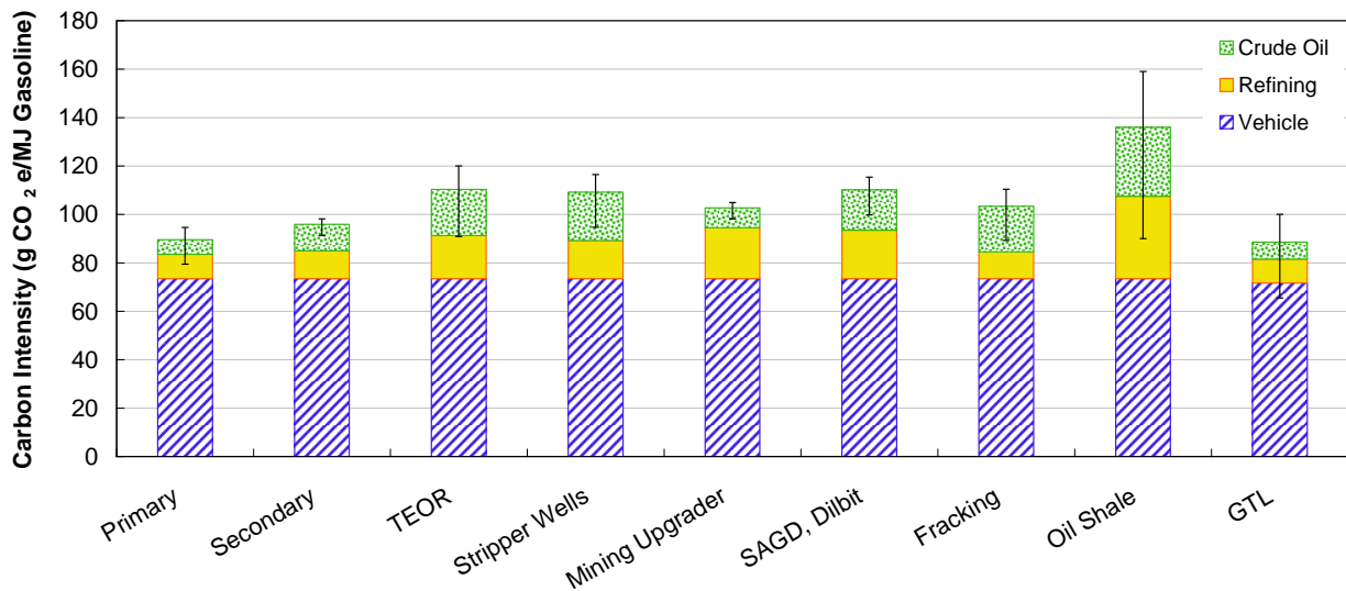
Figure 3.3. CI of gasoline emissions (g CO 2 e/MJ) from various petroleum production options.
