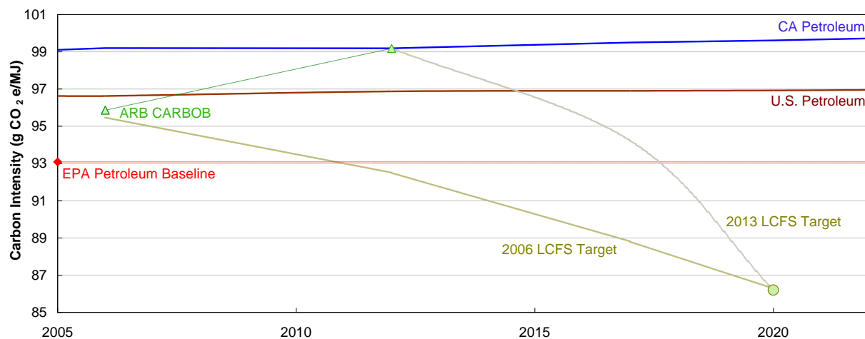
Figure 3.10. Weighted carbon intensity (g CO 2 e/MJ) of petroleum fuels consumed in the U.S. and California
