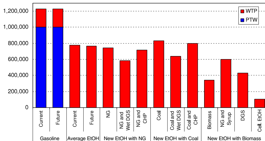
Figure 6. Well-to-wheels fossil energy use of ethanol and gasoline (Btu per million Btu of fuel produced and used).
